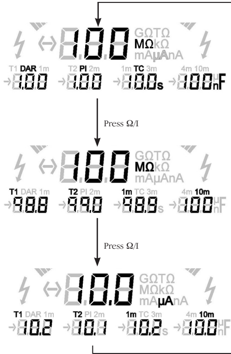
Figure 2 - The result of a polarity index test (PI)
