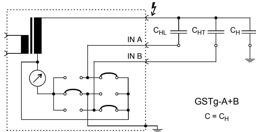
Figure 5-26 Measurement of C_H in GST-gA+B mode, C_{HL} and C_{HT} are guarded
