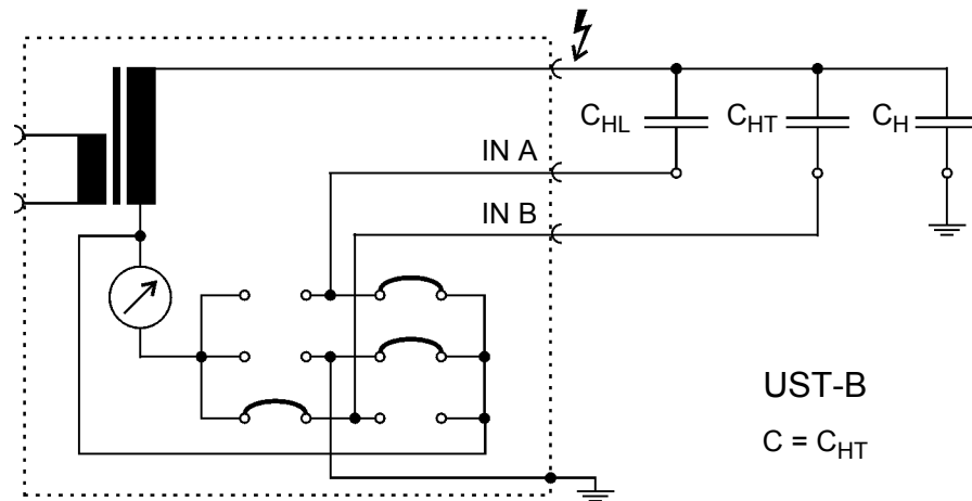
Figure 5-25 Measurement of C HT in UST-B mode, C HL and C H are guarded
