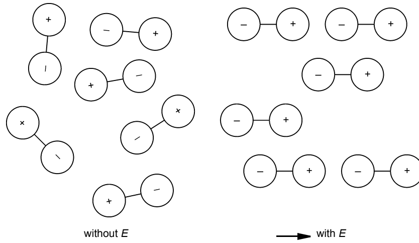
Figure 5-7 Polarization of dipoles in the electrical field
