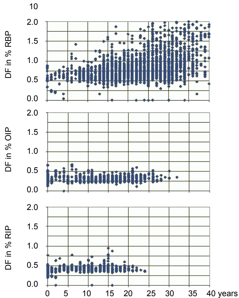
Figure 12-34 Aging of RBP, RIP and OIP bushings (change of DF)
