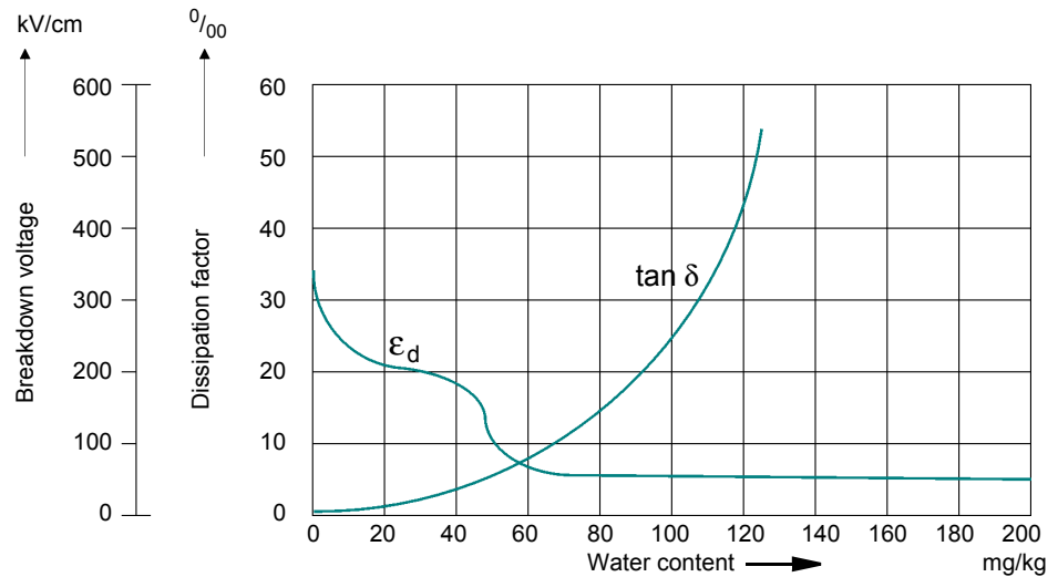
Figure 5-10 Breakdown voltage and DF in oil, dependent on the water content
