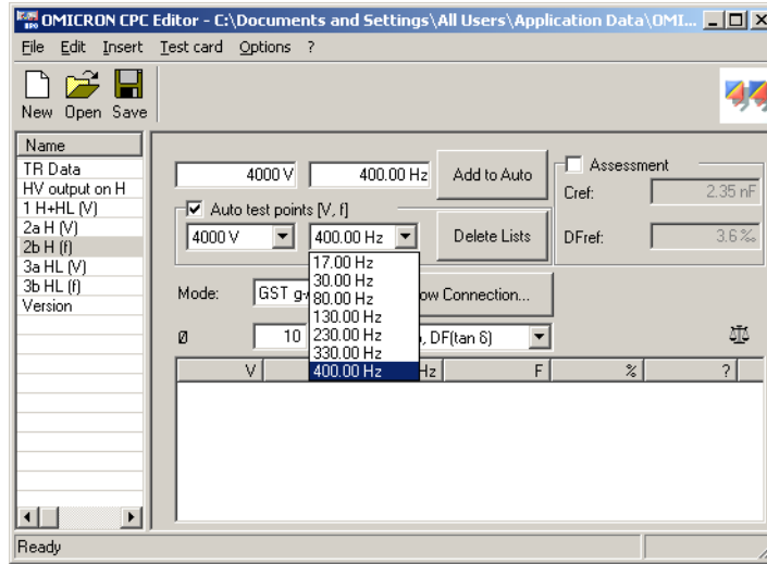
Figure 6-9 Frequency-scan of high-voltage windings to tank and core (GST gA+B)
