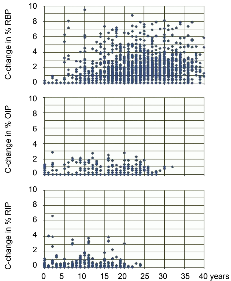
Figure 12-33 Aging of RBP, RIP and OIP bushings (change of capacitance) [10]
