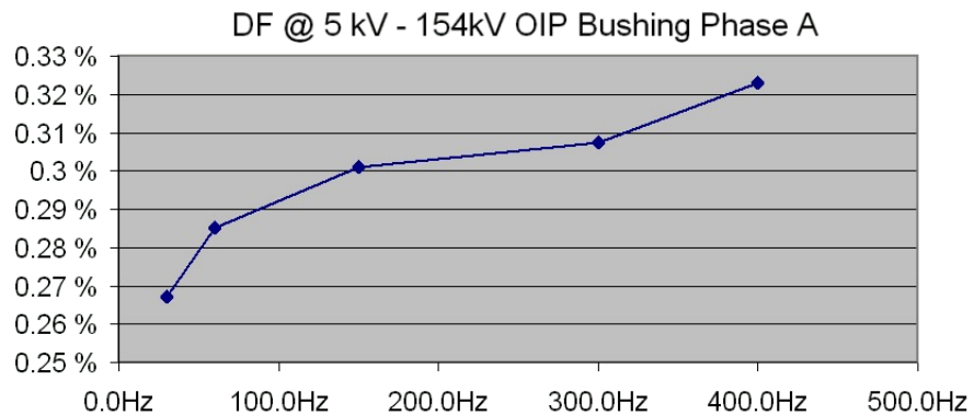
Figure 12-37 DF of an OIP 154 kV bushing (1970)
