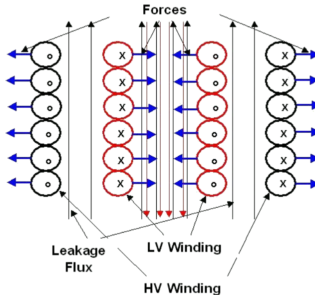
Figure 12-23 Leakage flux and forces during a fault
