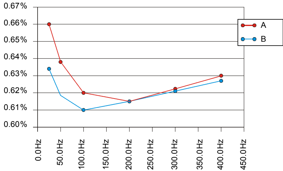
Figure 7-9 Frequency scan of an aged RIP bushing
