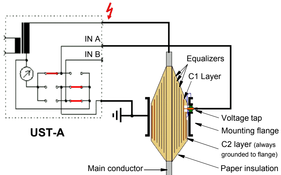
Figure 7-4 UST bushing test (C1)
