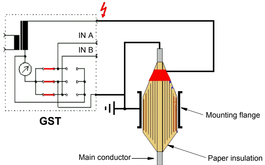
Figure 7-6 Bushing "hot collar" test
