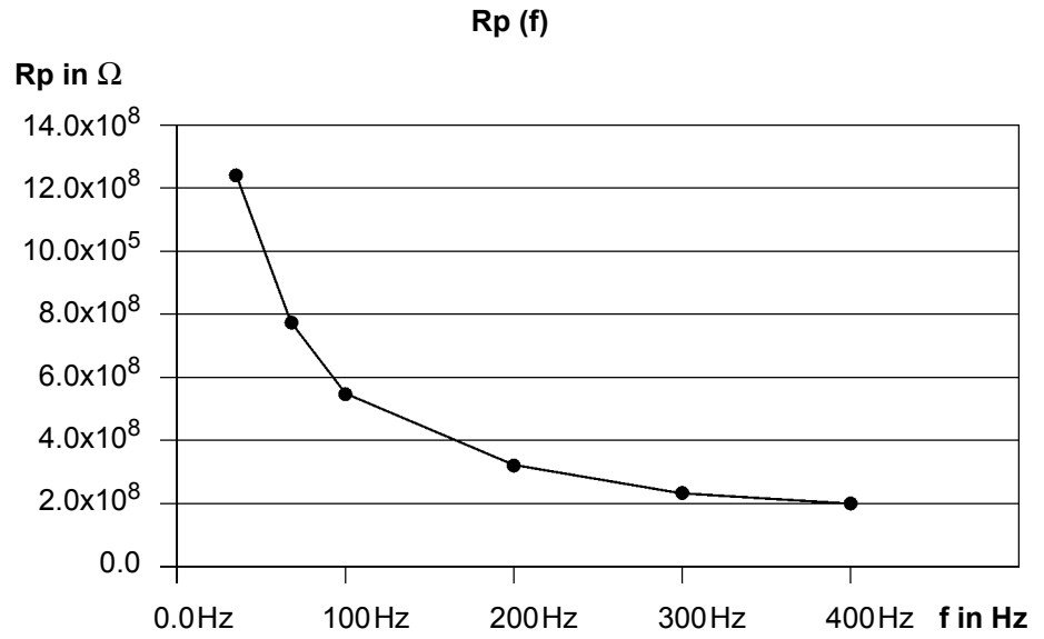
Figure 10-3 Lightning arrester Rp (f)
