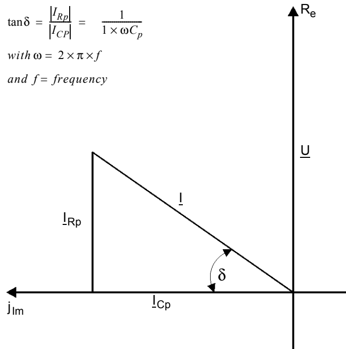
Figure 12-27 Definition of dissipation factor ( \tan \delta ) and the vector diagram
