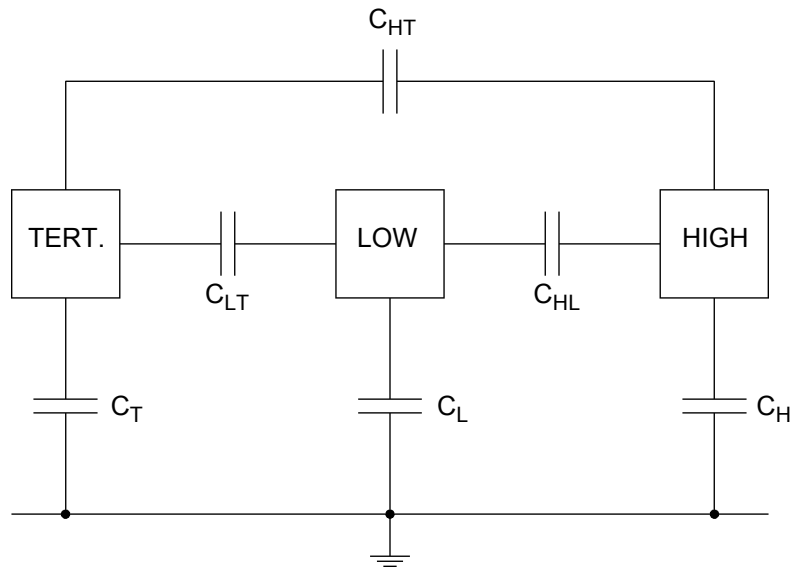
Figure 6-4 Three-winding transformer test according to IEEE 62-1995
