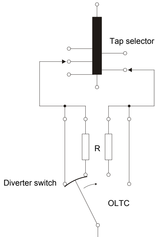
Figure 12-9 Equivalent circuit diagram of On-Load Tap Changer (OLTC)
