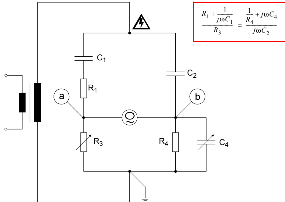
Figure 5-18 Schering bridge
