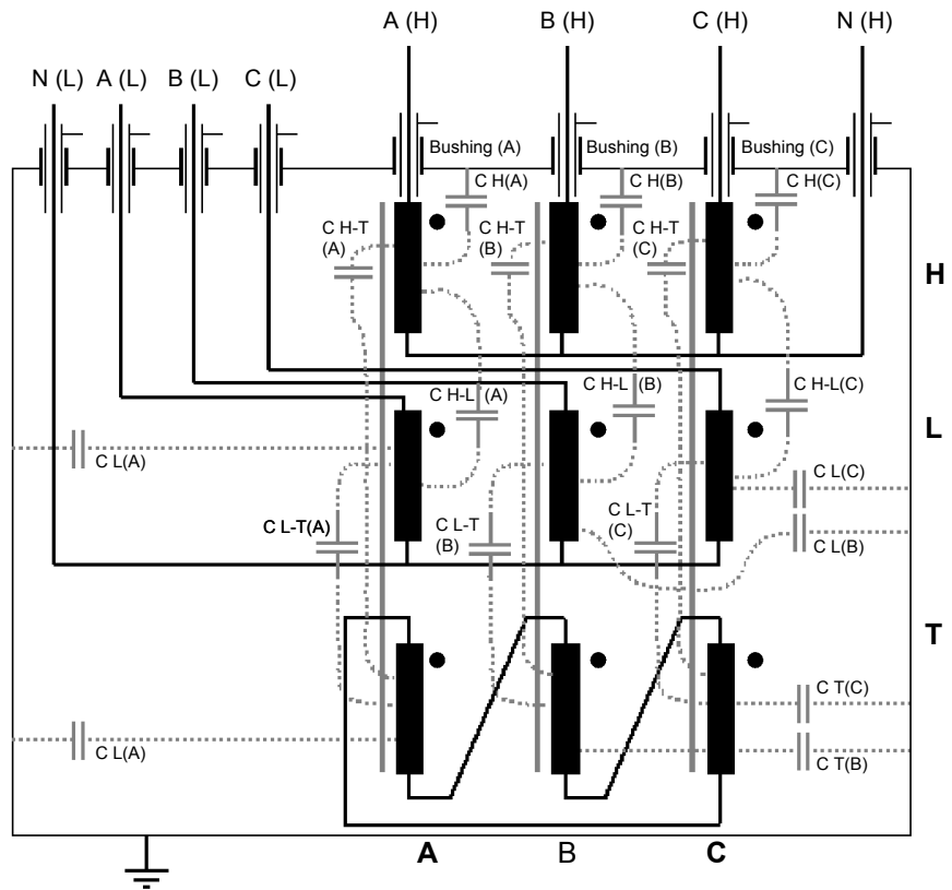
Figure 6-2 Three-winding transformer with winding to winding and winding to ground capacitors
