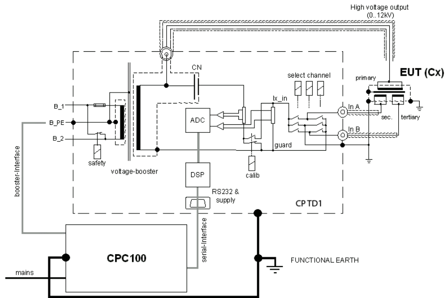
Figure 5-20 CP TD1 measuring principle
