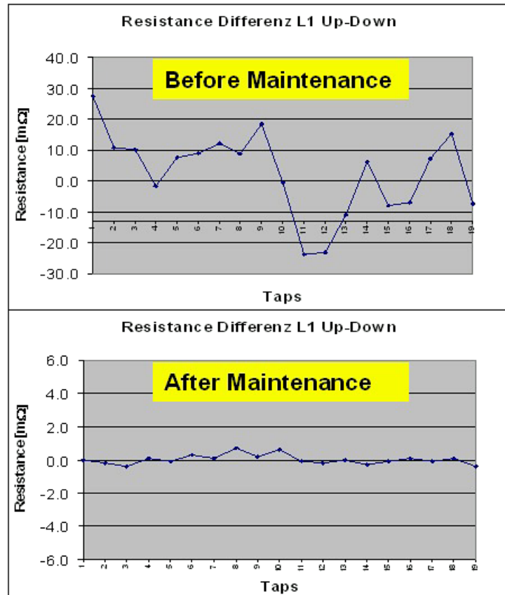
Figure 12-19 Difference "UP" - "DOWN"
