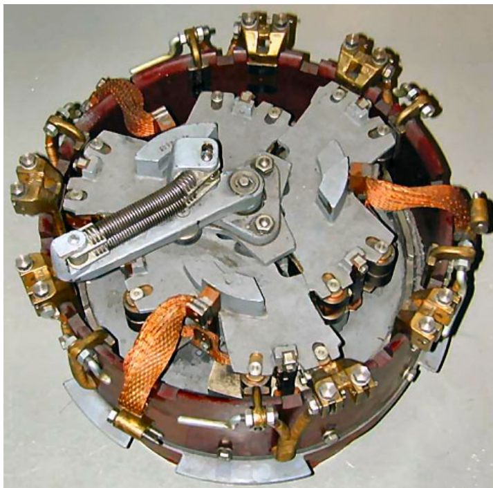
Figure 12-12 Diverter switch for 110 kV/40 MVA
