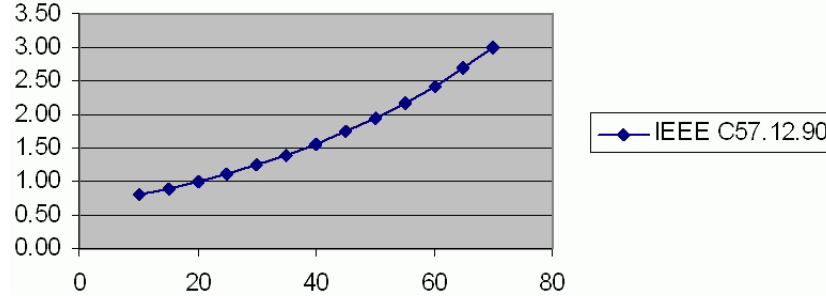
Figure 5-12 Temperature correction factor for mineral oil insulation [2.4]
