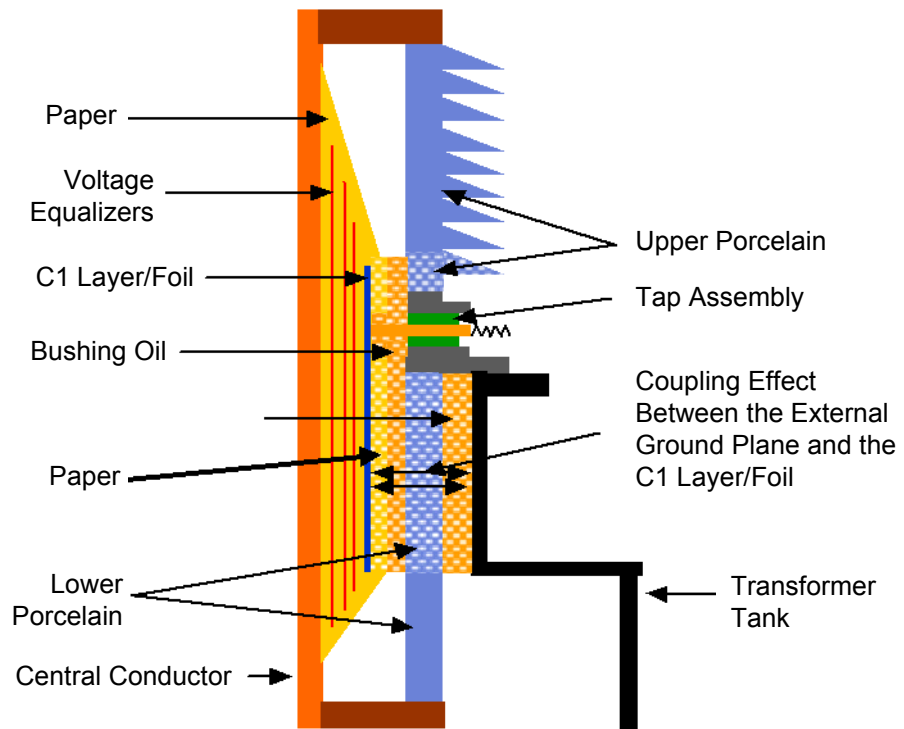
Figure 12-4 Design/construction details of a typical high current type T bushing and the influence of surrounding materials/objects
