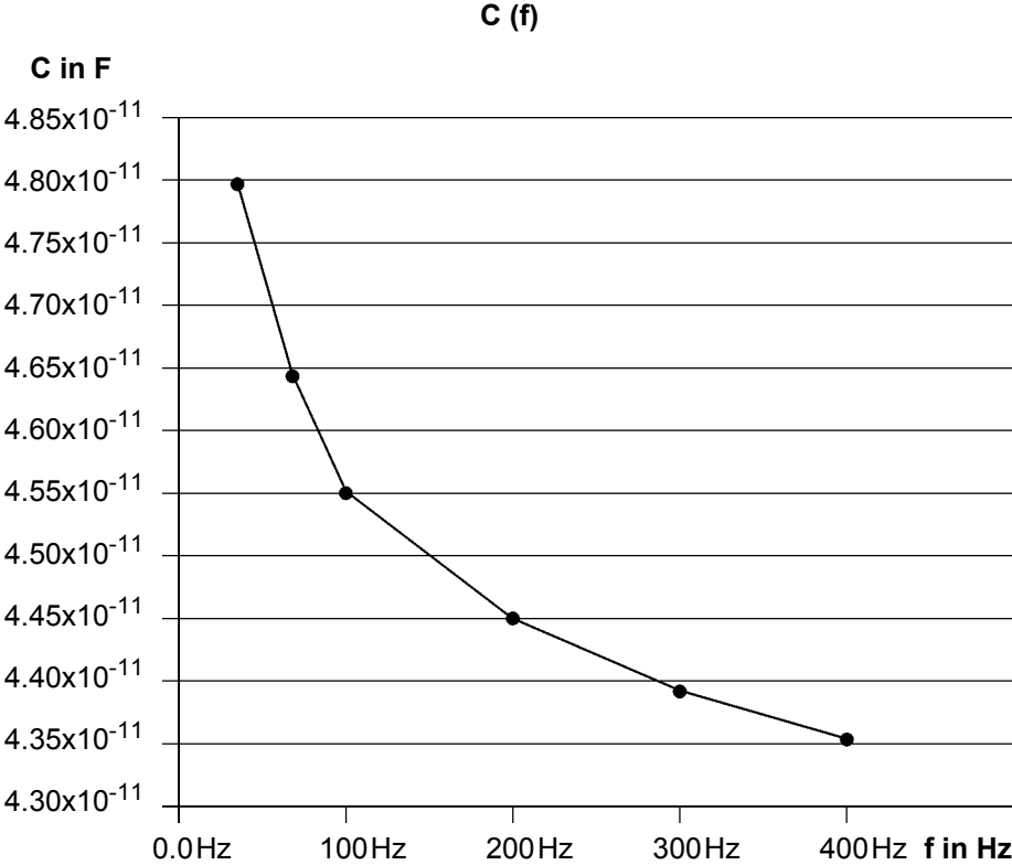
Figure 10-2 Lightning arrester C (f)
