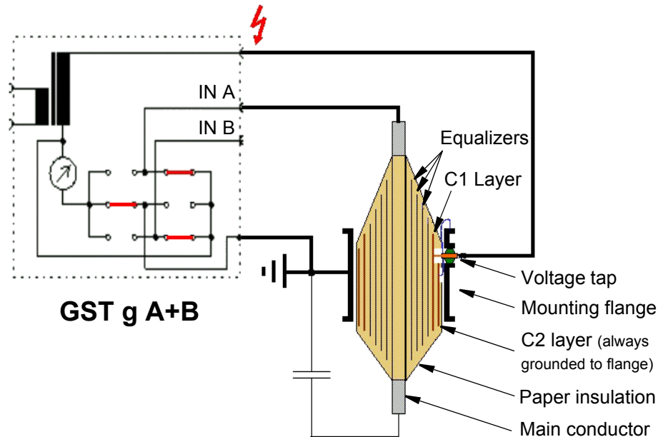
Figure 7-5 GST bushing test (C2)
