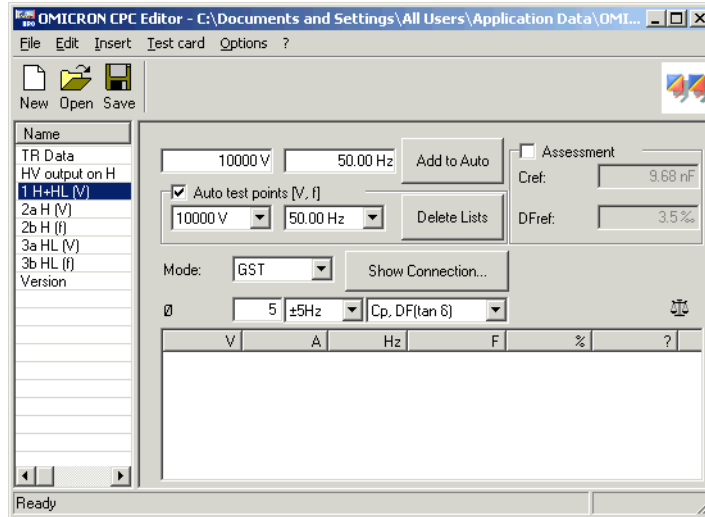
Figure 6-7 Measurement of C H and C H-L in GST g-B mode
