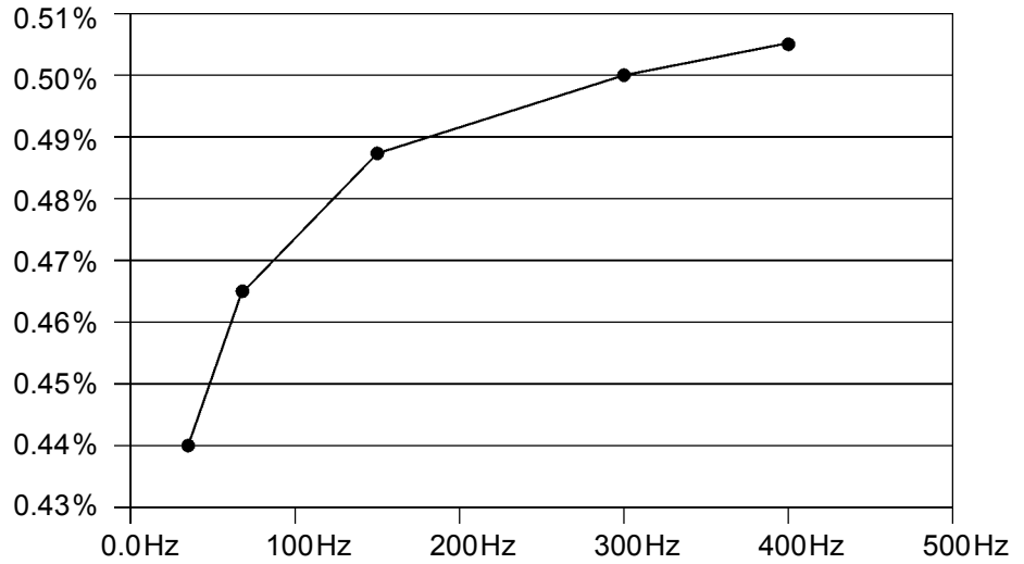
Figure 7-9 Frequency scan of an aged RIP bushing
