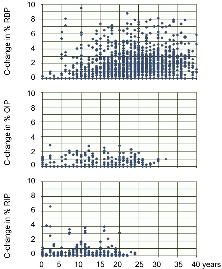
Figure 7-11 Aging of RBP, RIP and OIP bushings (change of capacitance)
