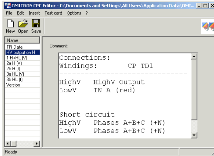
Figure 6-17 Two-winding transformer test preparation with CPC Editor
