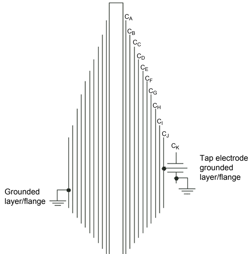
Figure 7-2 Condenser bushing design [4.1]
