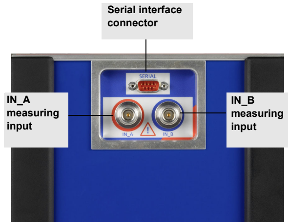
Figure 1-3 Serial interface and measuring inputs of the CP TD1
