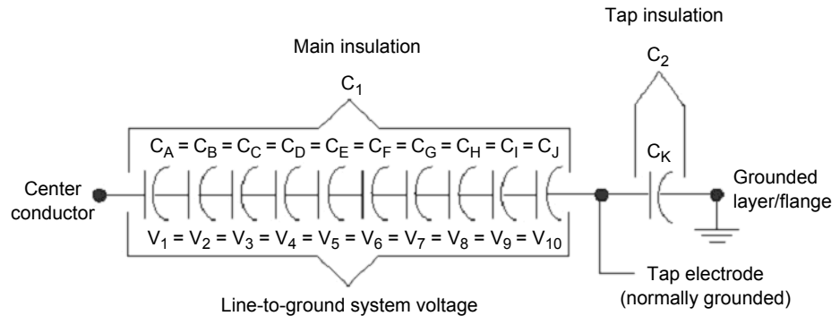
Figure 7-3 Condenser bushing circuit diagram [4.1]
