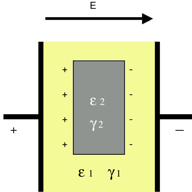
Figure 5-9 Interfacial polarization
