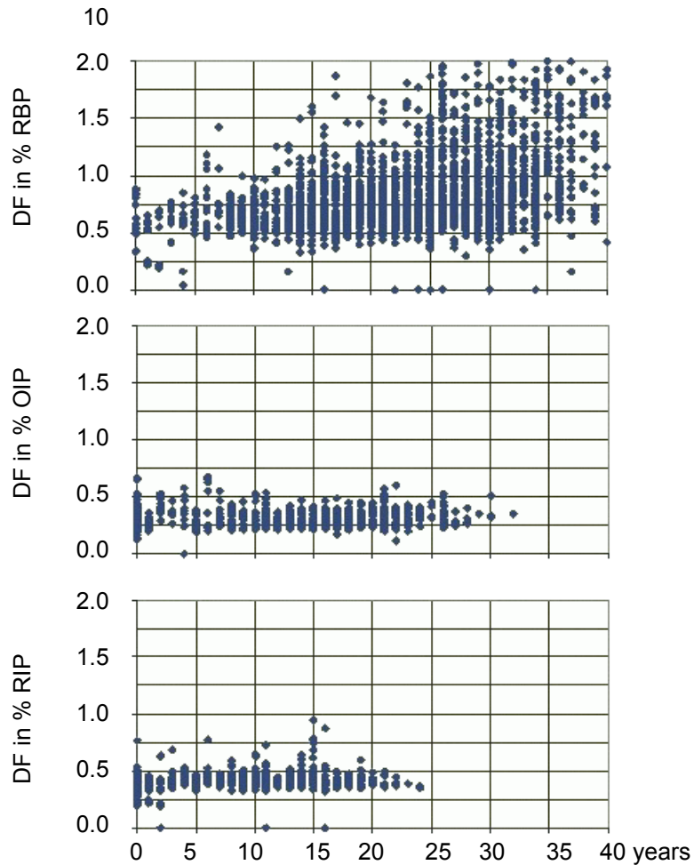
Figure 7-12 Aging of RBP, RIP and OIP bushings (change of DF)
