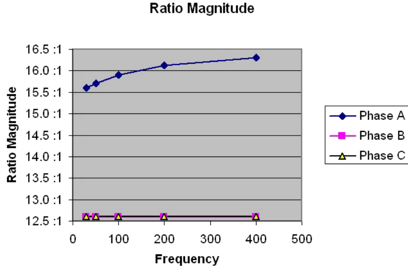
Figure 12-21 Ratio magnitude = f(f)
