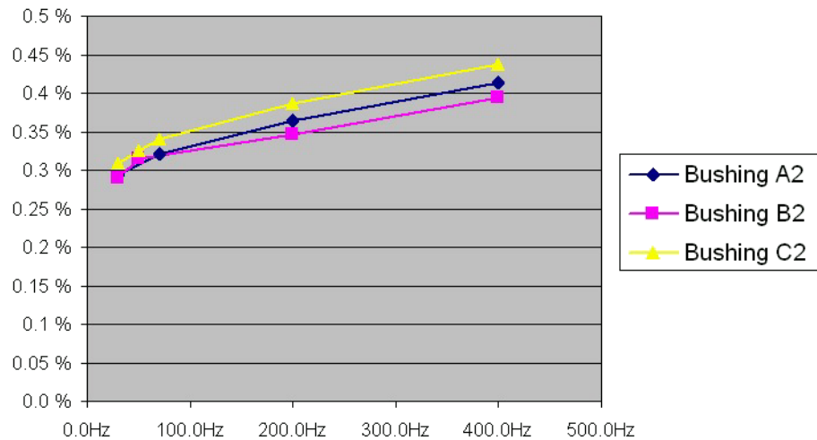
Figure 12-36 DF of a RIP 145 kV bushing (MICAFIL new)
