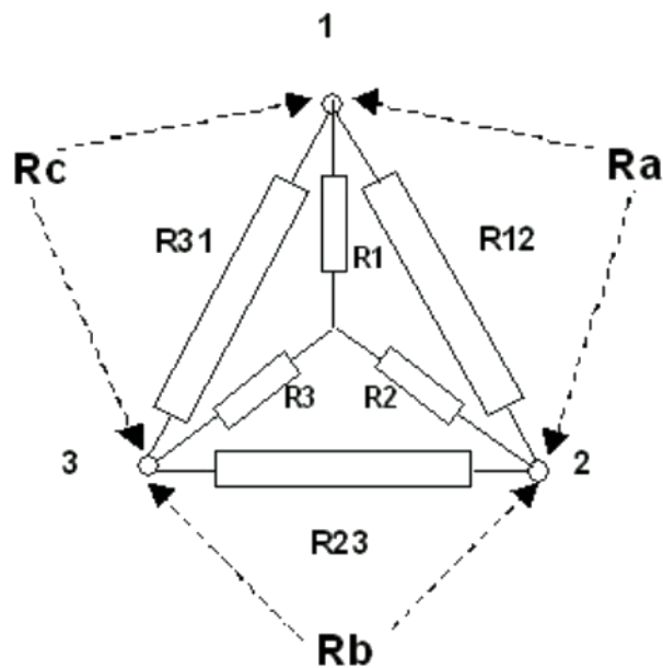
Figure 12-15 Delta-connected windings
