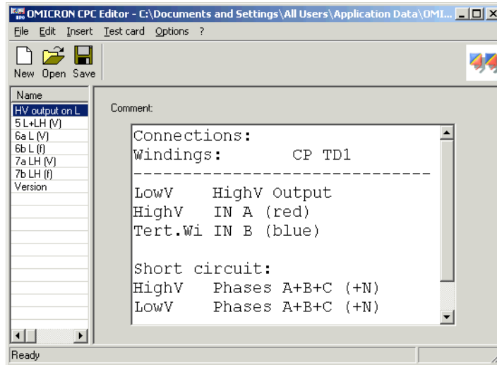
Figure 6-10 Connection instructions for the tests with energized low-voltage winding
