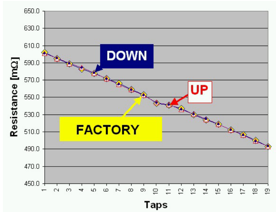
Figure 12-18 Resistance after maintenance
