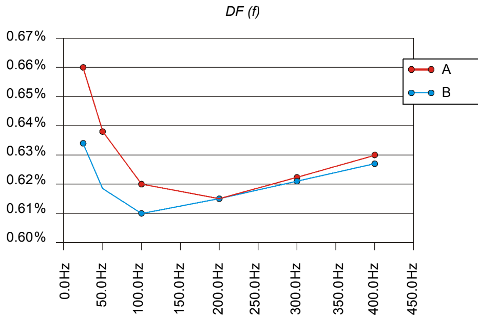
Figure 5-15 Frequency scan winding to winding DF measurement (oil-paper)
