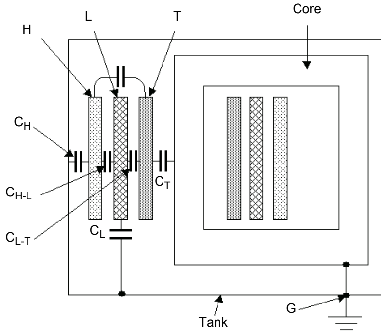
Figure 6-3 Three-phase transformer with winding capacitances
