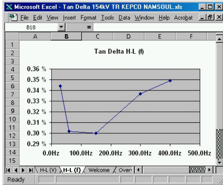
Figure 6-14 Frequency scan for H-L (f) (5 kV)
