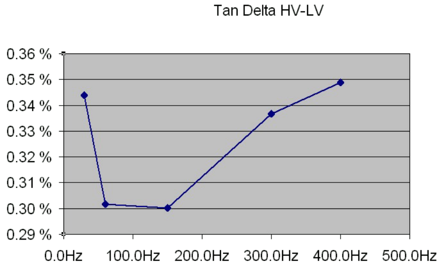
Figure 12-32 Frequency scan HV-LV (154 kV-20 kV)
