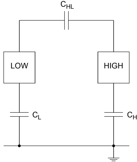
Figure 6-16 Two-winding transformer test according to IEEE 62-1995
