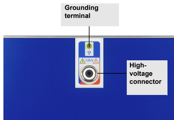
Figure 1-4 High-voltage connector of the CP TD1
