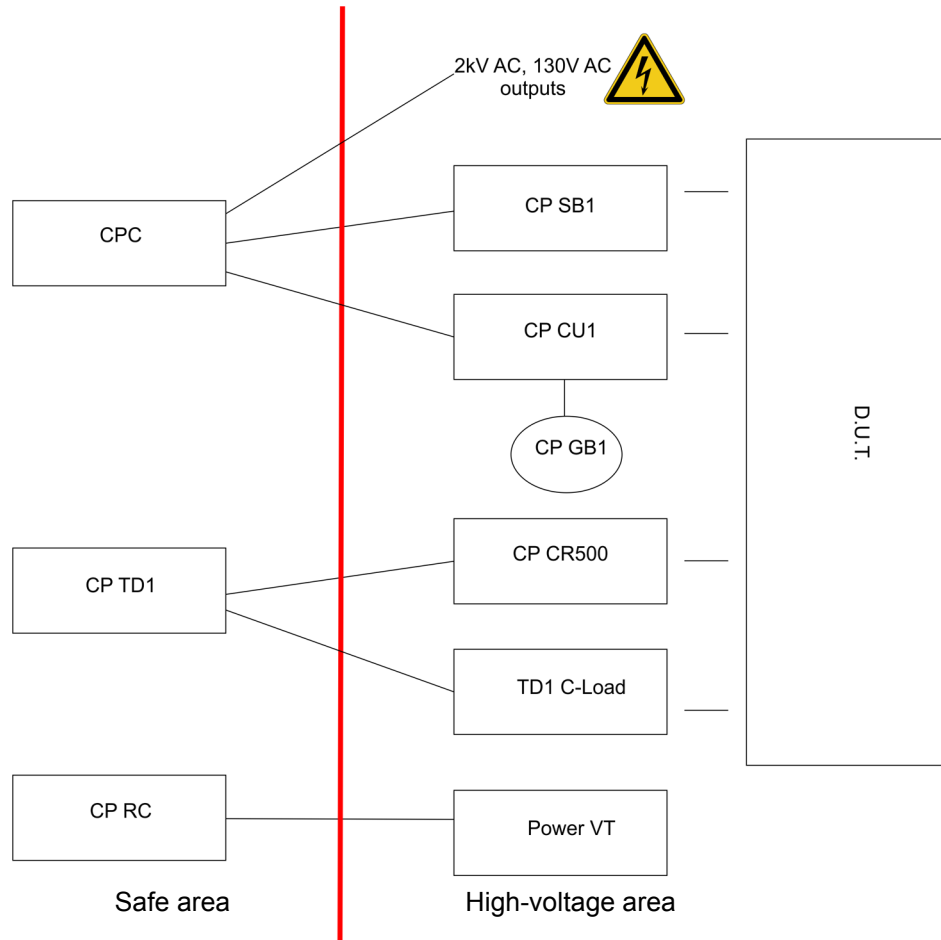
Figure 1-1 Example for the separation of safe and high-voltage area using different OMICRON electronics devices
