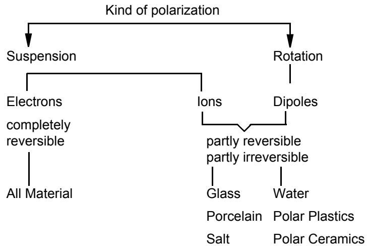
Figure 5-4 Kind of polarization
