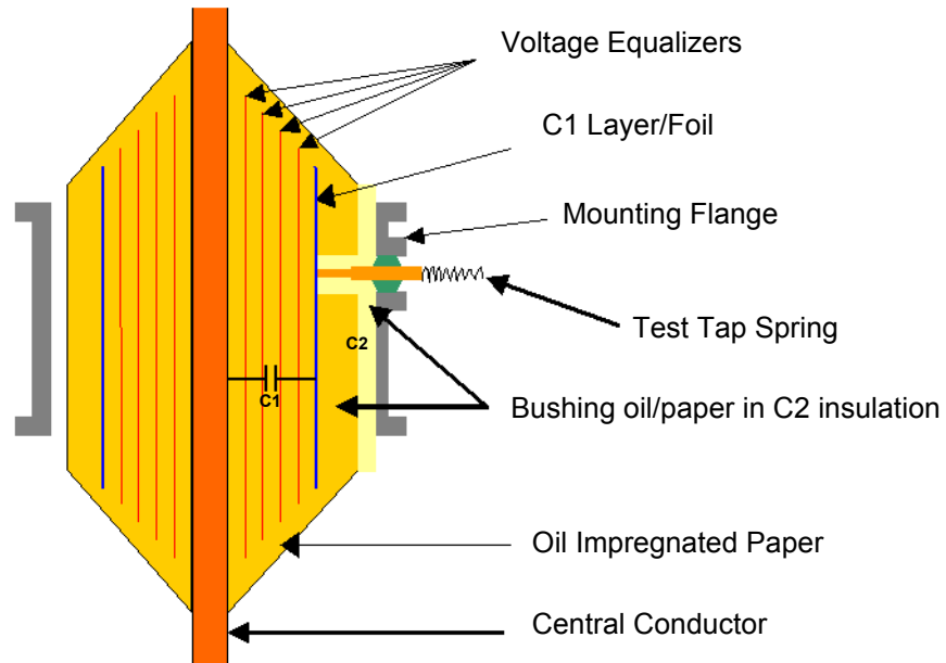
Figure 12-3 Design/construction details of a typical condenser bushing rated 69 kV and below
