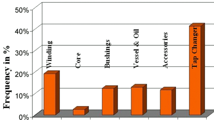
Figure 12-7 Sources of transformer faults
