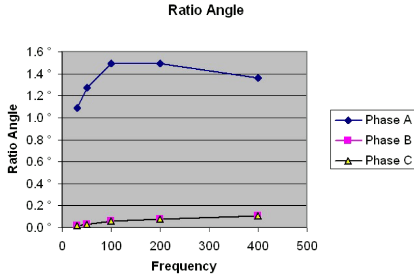
Figure 12-22 Ratio phase angle = f(f)
