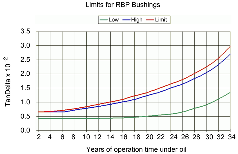
Figure 7-13 Limits for RBP bushings
