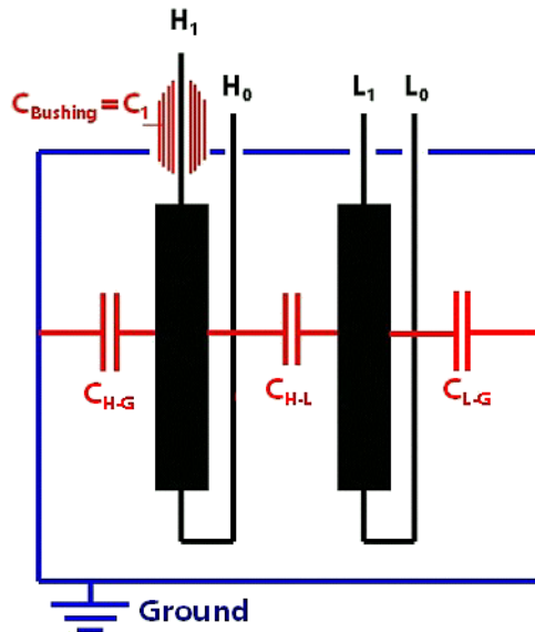
Figure 12-31 2-winding transformer
