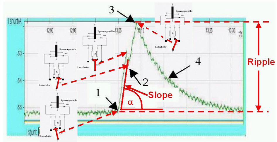
Figure 12-20 Dynamic resistance measurement for analysis of the diverter switch
