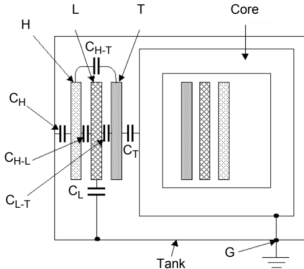
Figure 5-21 Three-phase transformer with winding capacitances
