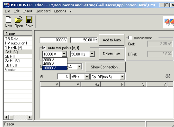
Figure 6-8 Voltage-scan of high-voltage windings to tank and core (GST gA+B)
