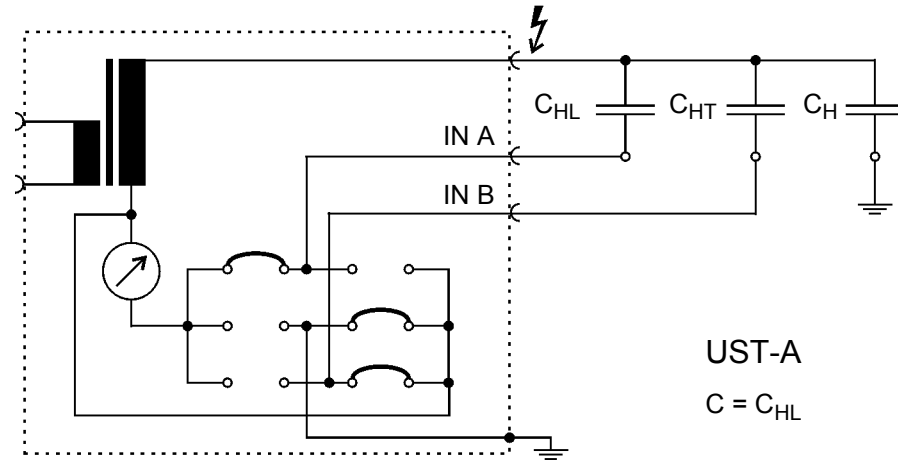
Figure 5-24 Measurement of C_{HL} in UST-A mode, C_{HT} and C_H are guarded
