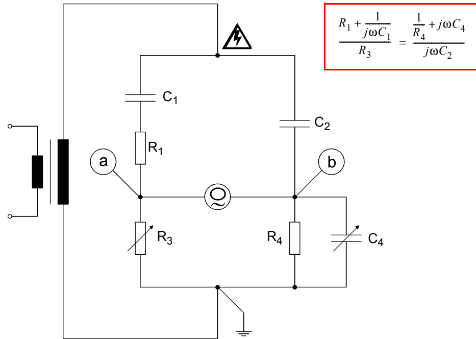
Figure 12-28 Schering bridge
