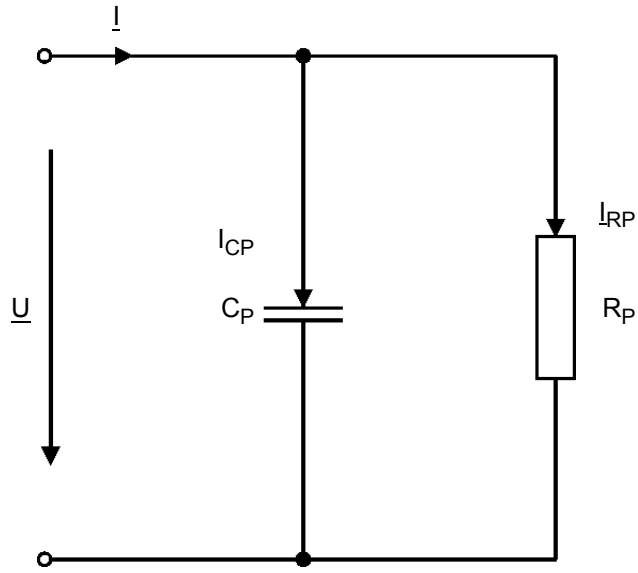
Figure 5-1 Simplified circuit diagram of a capacitor
