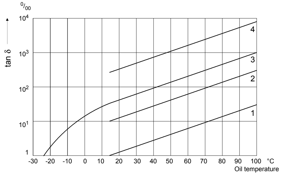
Figure 5-11 DF of new and aged oil, dependent on temperature
