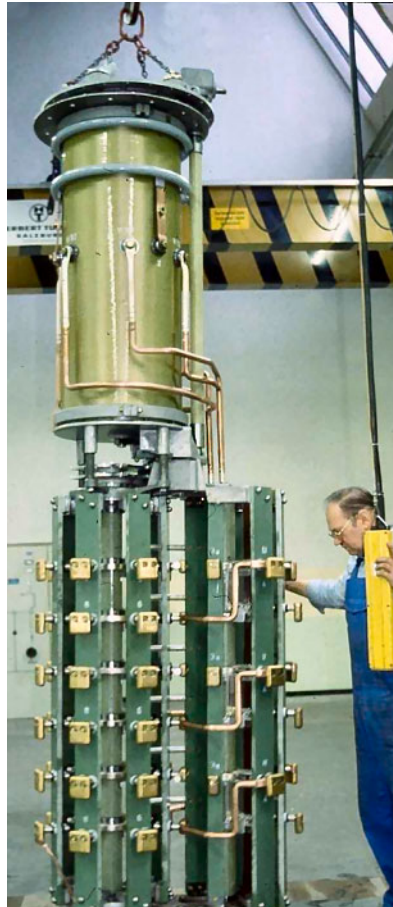
Figure 12-10 Tap changer
