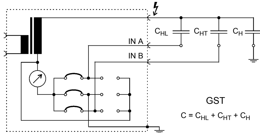
Figure 5-23 CP TD1 block diagram of GST mode
