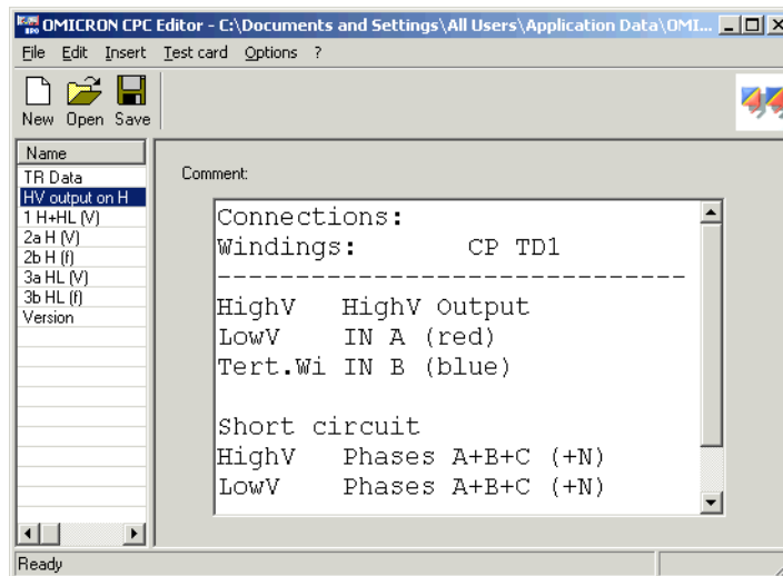
Figure 6-6 Instruction about test lead connections
