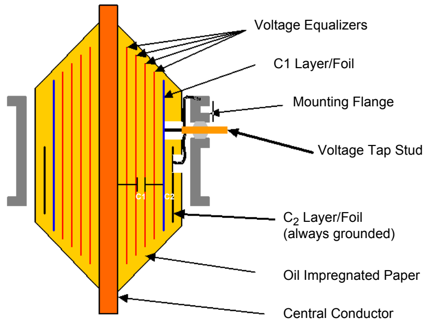
Figure 12-2 Design/construction details of a typical condenser bushing rated 115 kV and above
