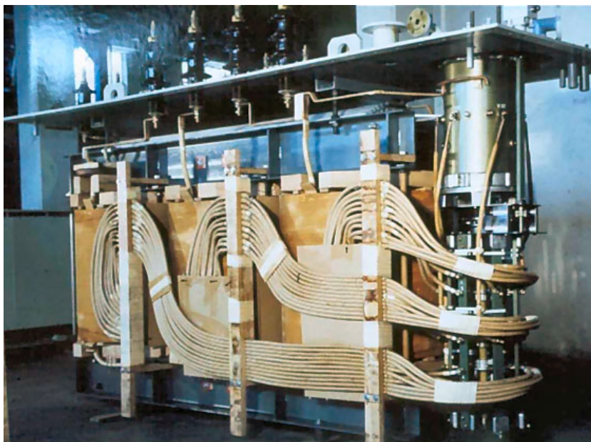
Figure 12-11 Transformer with tap changer
