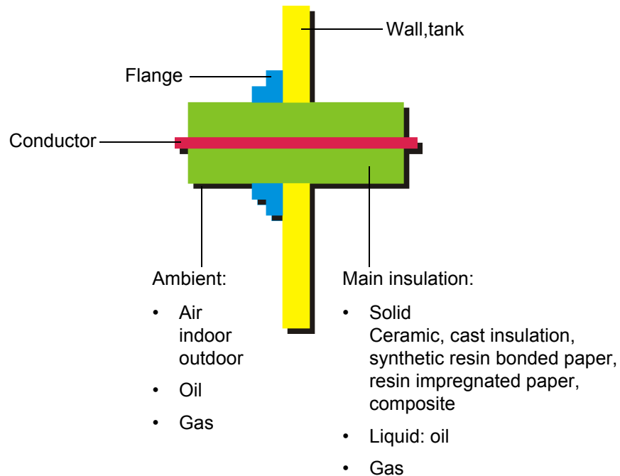
Figure 7-1 Principle of bushings
