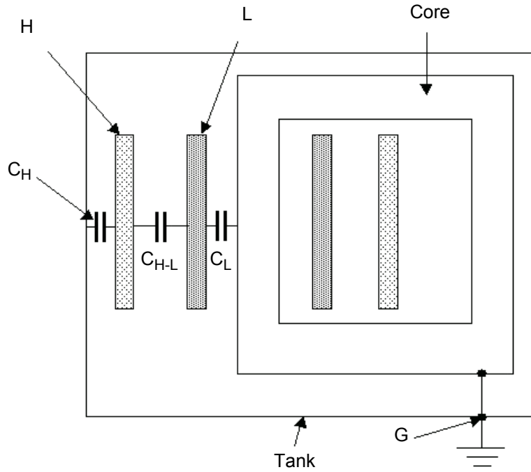
Figure 6-15 Two-winding transformer with winding capacitances
