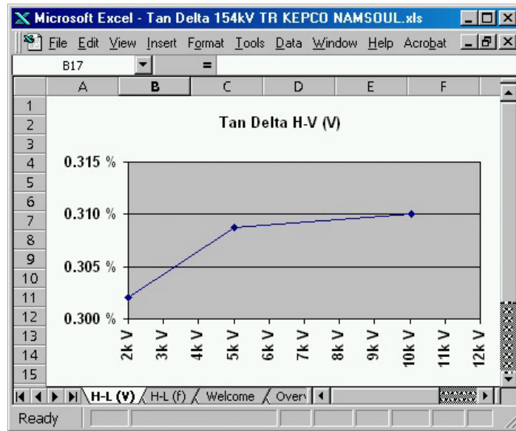
Figure 6-13 Voltage-scan for H-L (V) (50 Hz)
