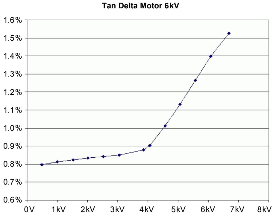
Figure 8-1 DF tip-up curve
