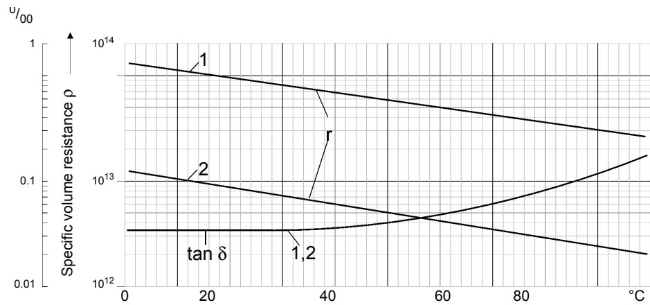
Figure 5-13 Temperature behavior of silicon liquid [2.3]
