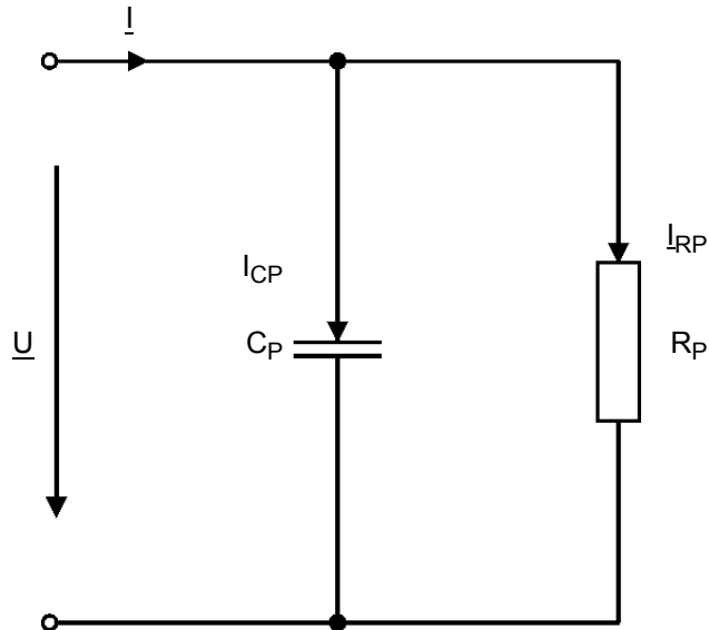
Figure 12-26 Simplified circuit diagram of a capacitor
