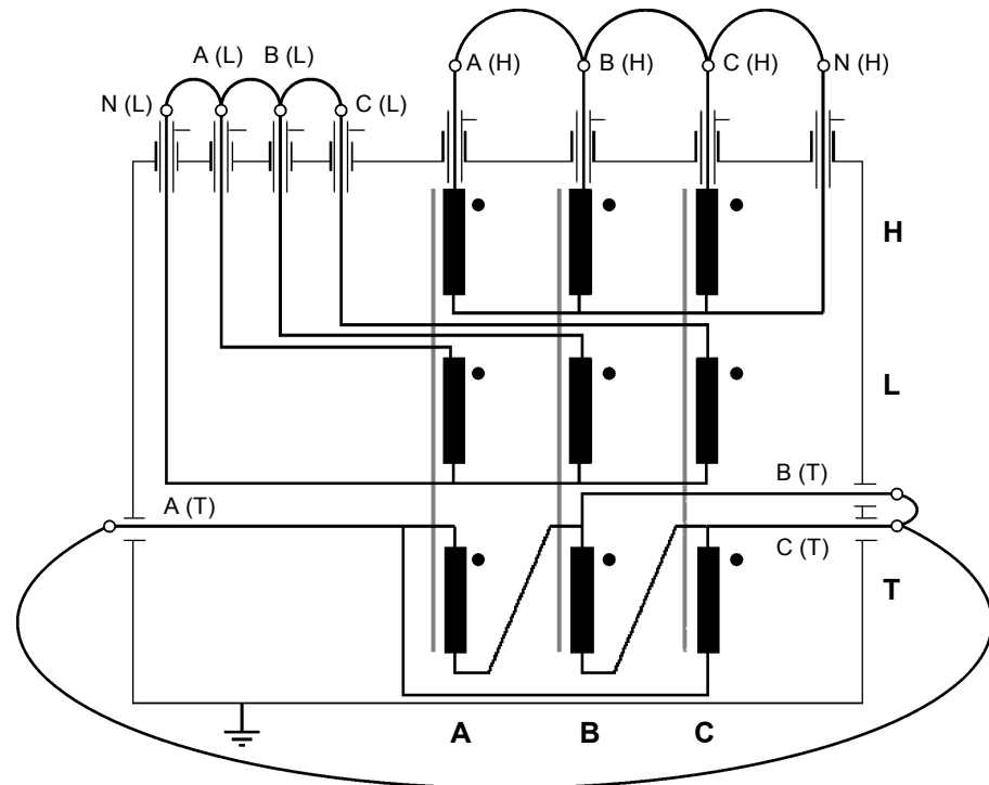
Figure 6-1 Three-winding transformer with connected winding
