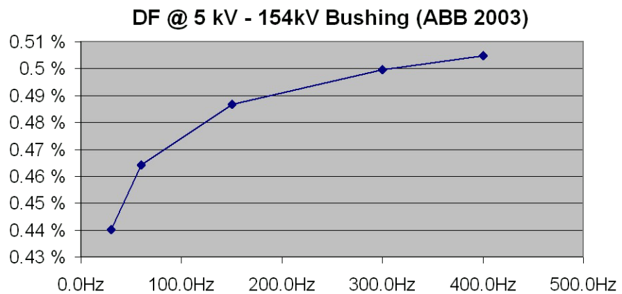
Figure 12-35 DF of a new 154 kV bushing
