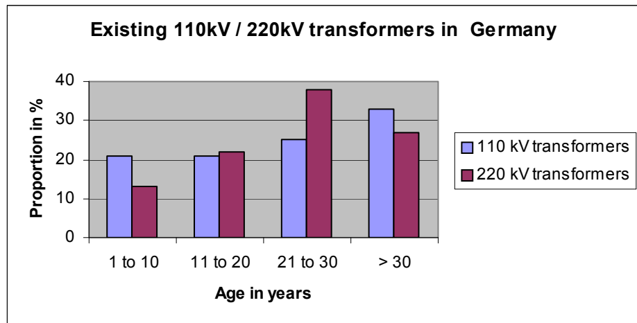
Figure 12-5 110/220 kV transformers in Germany
