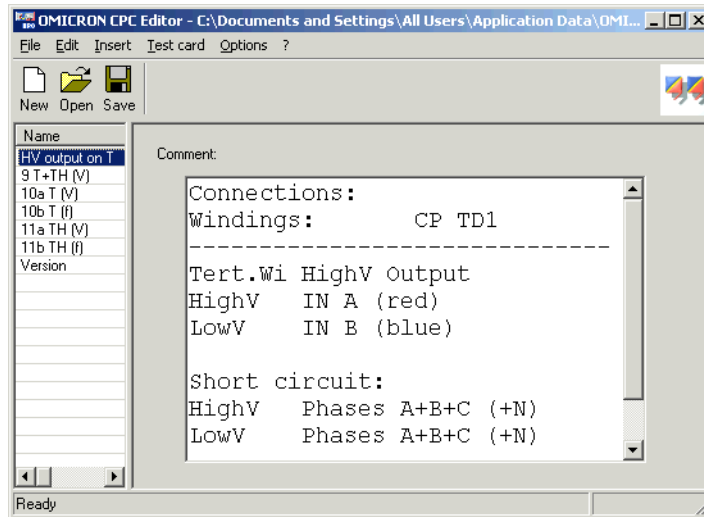
Figure 6-11 Connection instructions for the tests with energized tertiary winding
