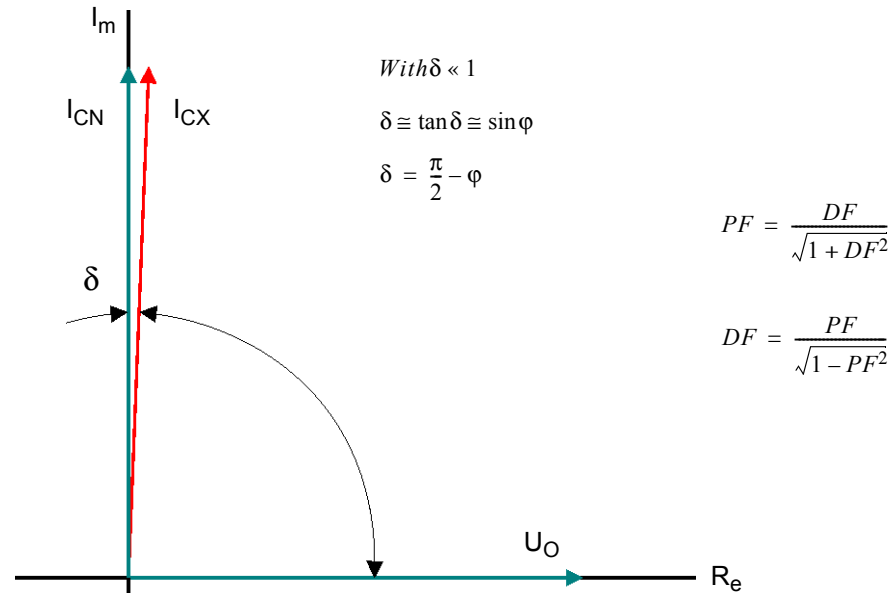
Figure 12-30 Correlation between DF and PF
