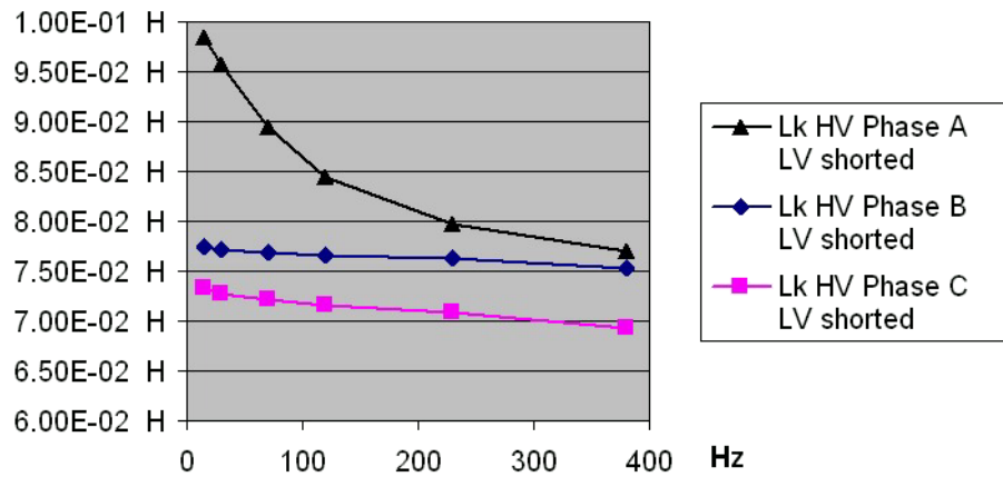
Figure 12-25 Leakage reactance frequency scan
