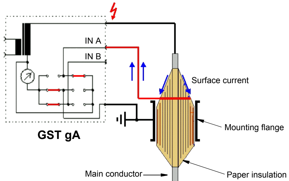
Figure 7-7 Use of guard method for bypassing the surface current
