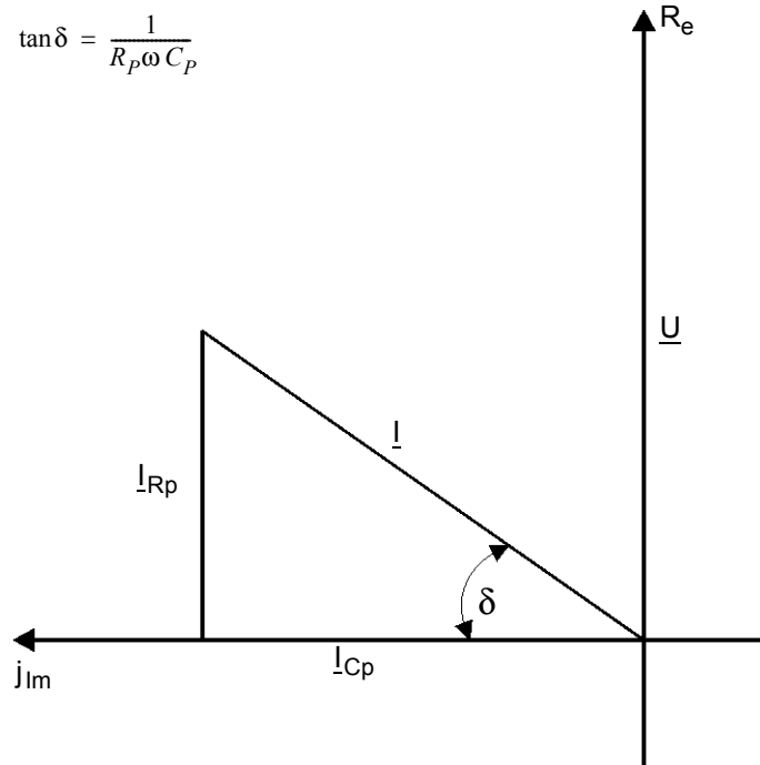
Figure 5-2 Definition of dissipation factor ( \tan \delta ) and the vector diagram
