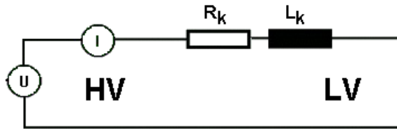
Figure 12-24 Short-circuit impedance test
