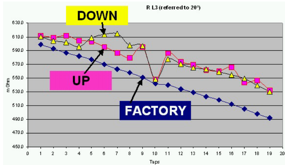
Figure 12-16 Winding resistance measurement H1-H0
