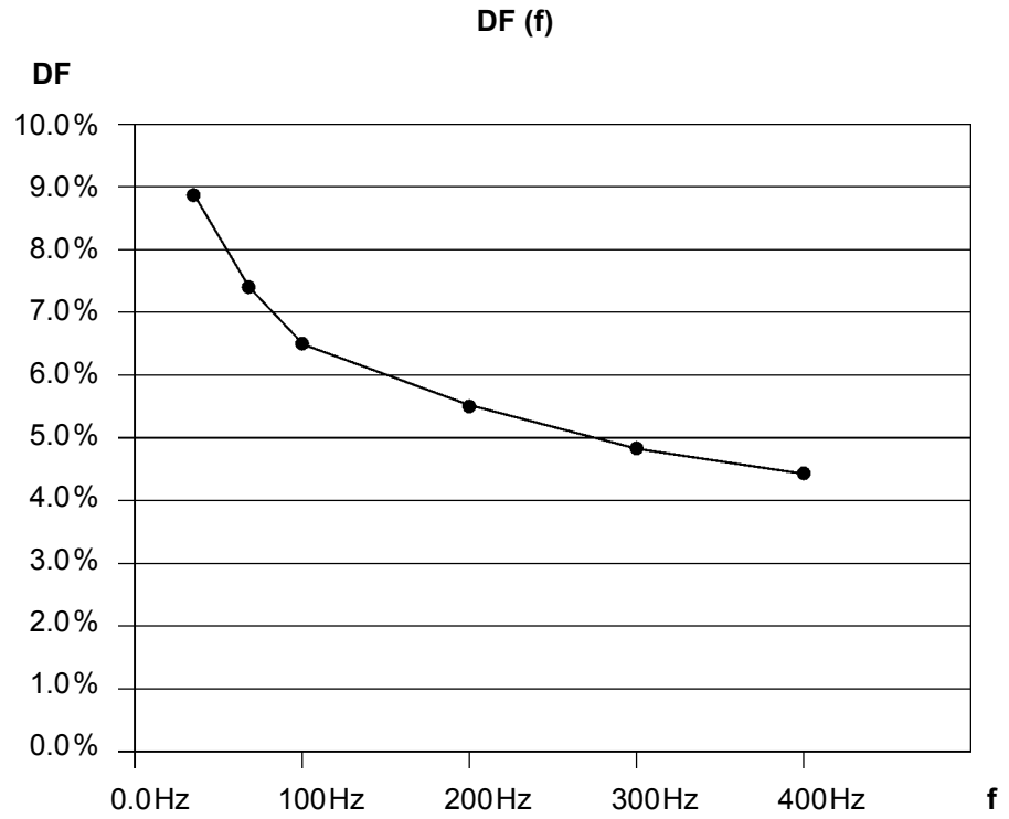
Figure 10-1 Lightning arrester DF (f)
