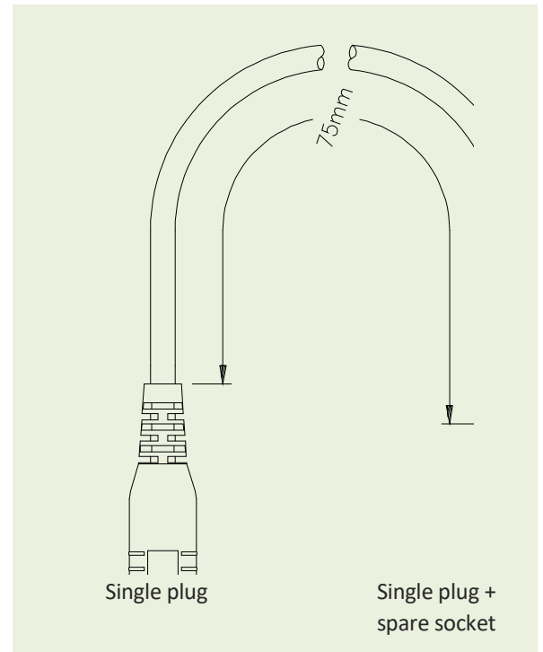
Figure 10: Two ended test lead – short - P/N 310-230-075-1
